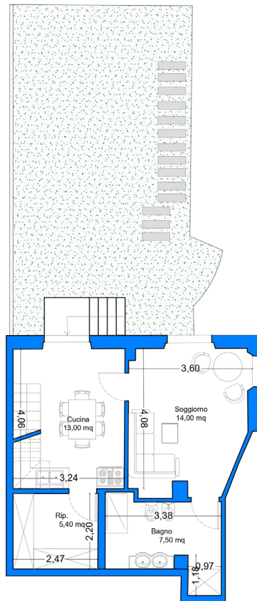
PIANO TERRA
